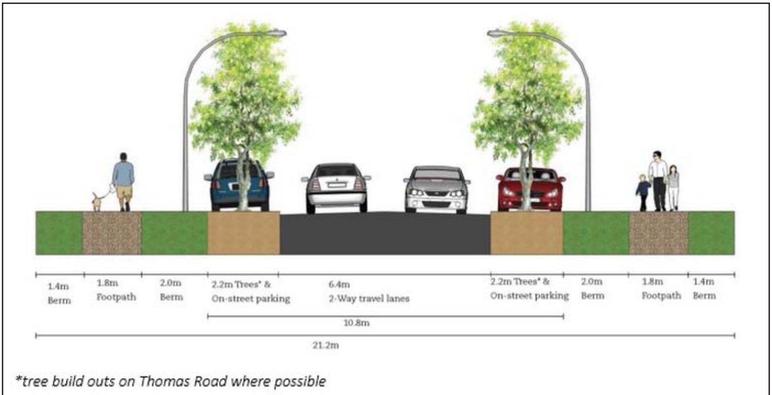
Figure 8. Collector Road Flat Bush sub-precinct C
